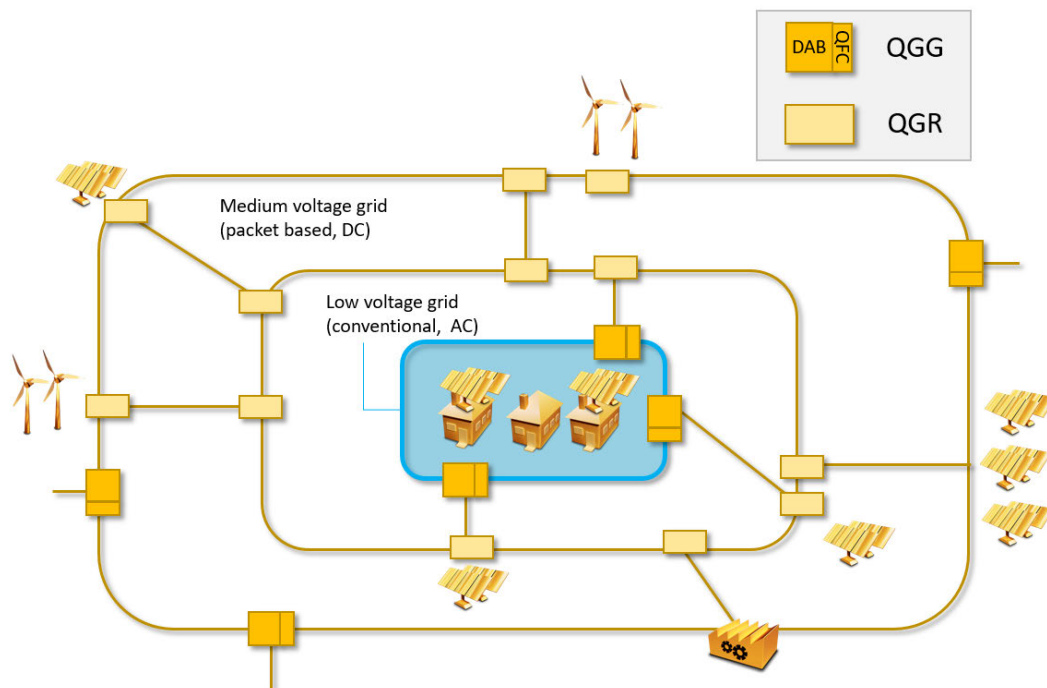
Fig. 25 The Quantum Grid Gateway (QGG) is the bridge between the traditional low voltage grid and the Quantum Grid at the medium voltage level. Both is possible: power flow control and voltage transformation.
