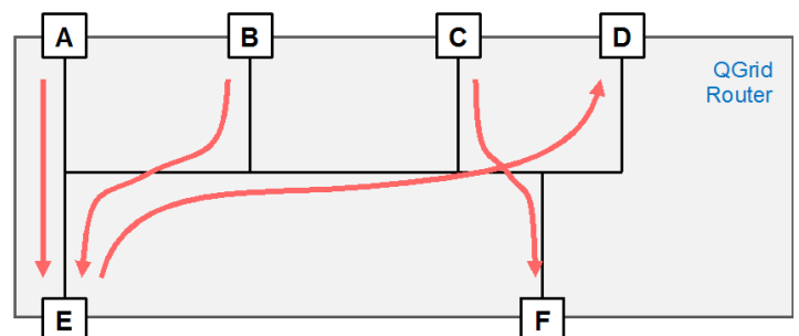
Fig. 16 Left: Order queue, which lists the energy packets that are sent from port to port within the QGR for each time interval. Right: QGR with six ports and power flows visualized by red arrows.
