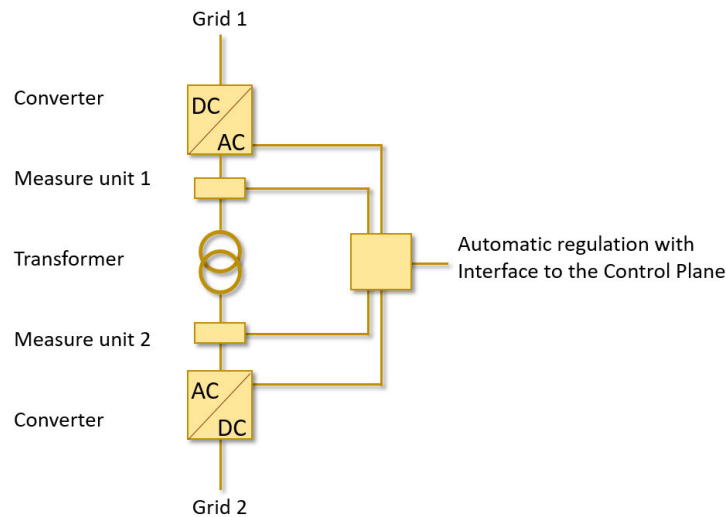
Fig. 20 Insight into a QFC: the DAB is responsible for the bidirectional DC/DC conversion.
