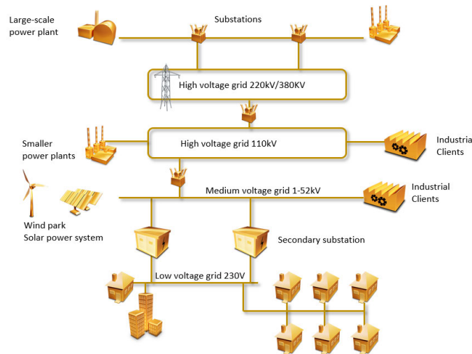
Fig. 24 Typical topology of the current electrical grid. The power flow is transformed from high voltage to medium voltage and finally down to low voltage at the customer side at transformer stations or substations.
