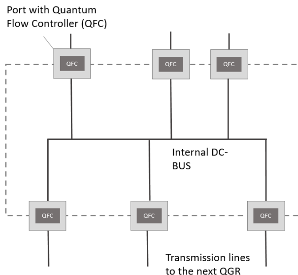
Fig. 7 Quantum Grid Router with six ports, each one containing a QFC. The QFCs are connected to the internal DC-bus.
