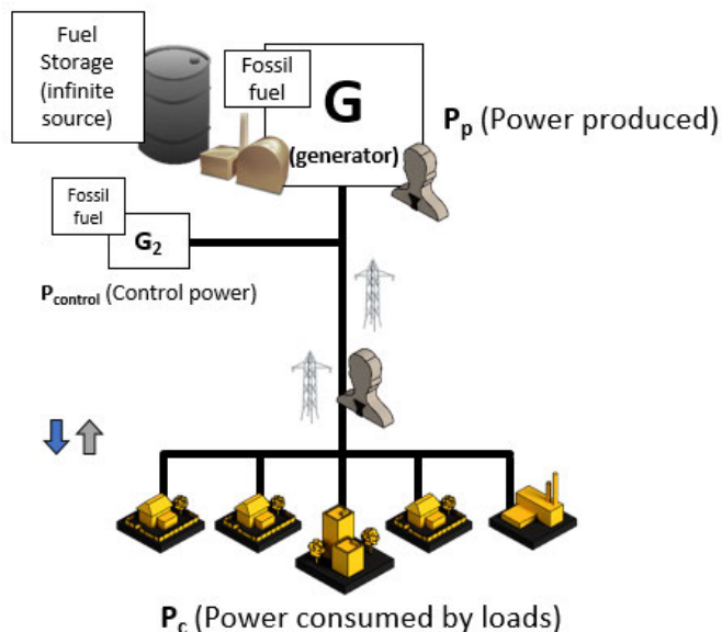
Fig. 1 Today's power on demand operation principle is only possible due to the usage of "unlimited" fossil fuel storage.
