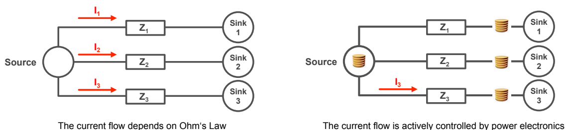
Fig. 6 Left: In a traditional grid, the power flows according to the laws of Kirchhoff and Ohm. Right: In the Quantum Grid, the power flow is controlled and forced to take a pre-determined way at each node in the grid by Quantum Grid Routers.
