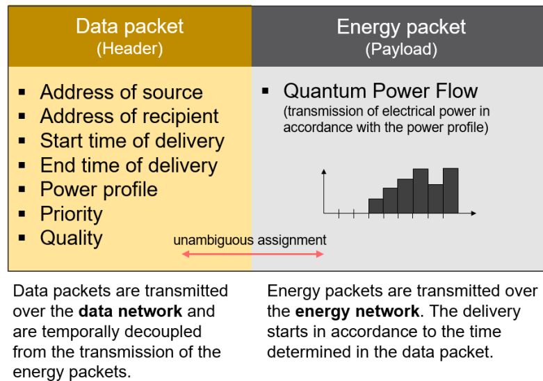
Fig. 5 Data packets and energy packets are unambiguously assigned to each other and are transported through different networks: power grid and telecommunication network.
